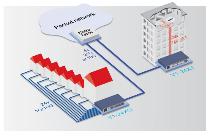
Typical applications with V1-24XG/XT
