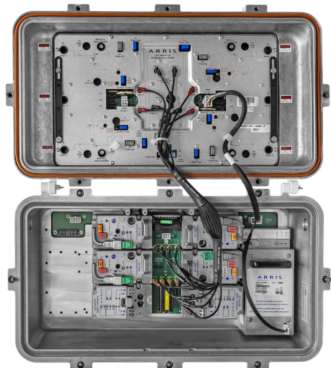
OM4120 with Deep Lid HFC Option
