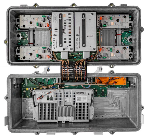
OM6000 with 1x1 RPD Module
