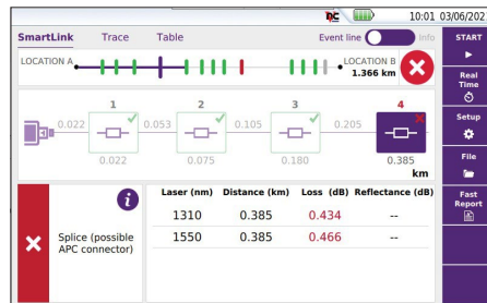
Smart Link Mapper view
