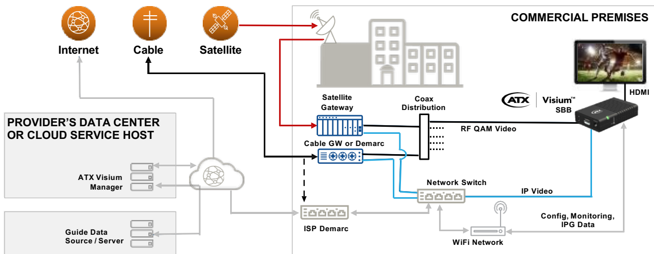
Application Diagram
